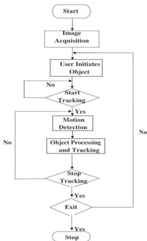
Fig. 1. Main program flow chart
